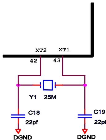
Figure 10-10 Crystal Circuit Diagram
