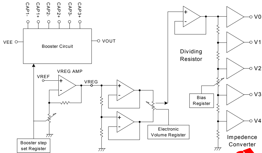
Figure 3. Power Circuit Block Diagram
