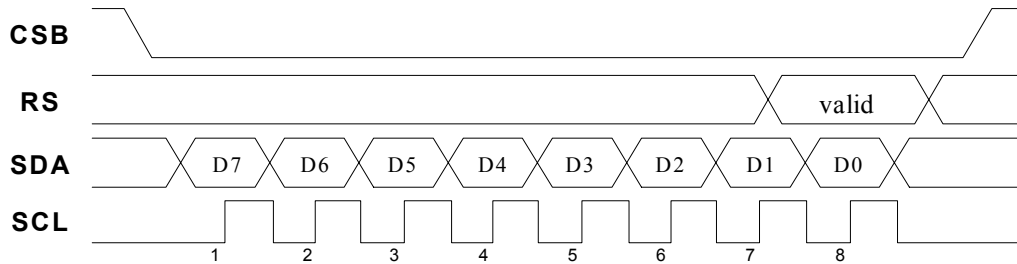
Figure 4. Serial Interface
