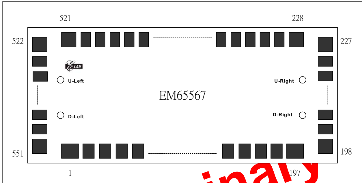
Figure 1. Pin configuration
