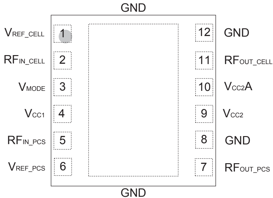
Figure 2: Pinout
