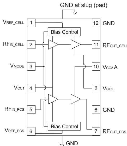
Figure 1: Block Diagram
