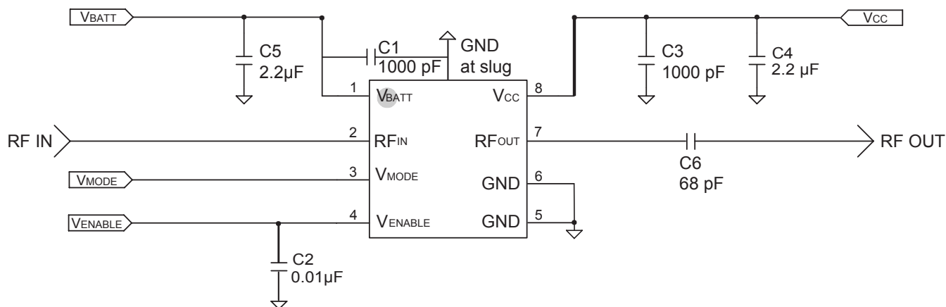
Figure 3: Application Circuit
