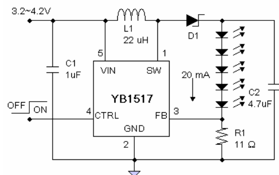
Figure 1 : White LED Driver
