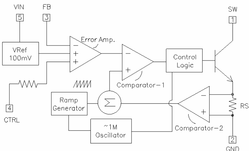
Figure 3: YB1517 Block Diagram
