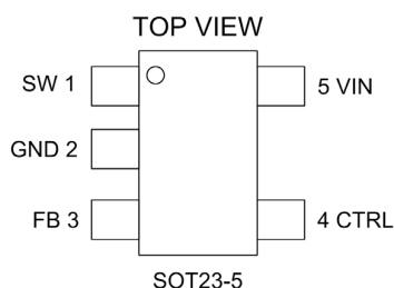
Figure 3 : YB1517 Pin Configuration
