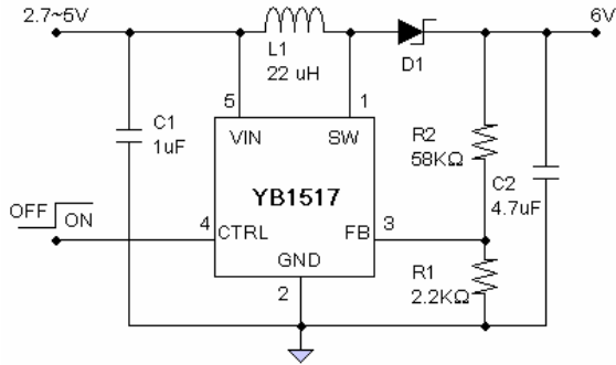
Figure 5 : TFT Panel Power Application Circuit
