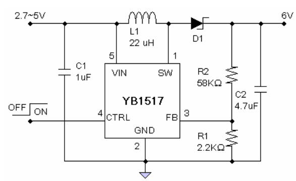
Figure 2 : DC-to-DC Converter
