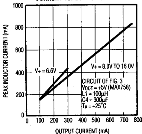
MAX738/MAX758 PEAK INDUCTOR CURRENT vs. OUTPUT CURRENT
