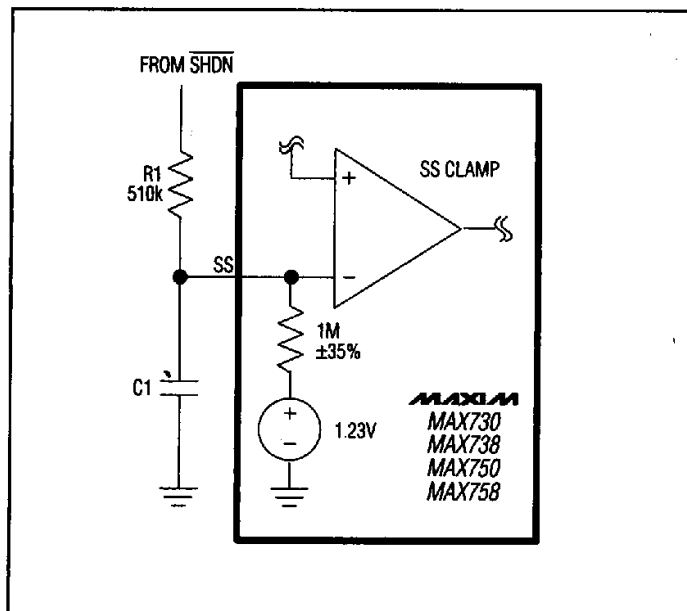
Figure 2. Block Diagram of Soft-Start Circuitry
