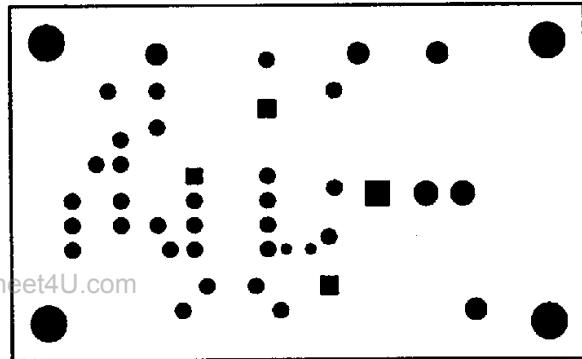
Figure 7. DIP PC Layout, Drill Guide (1X Scale)
