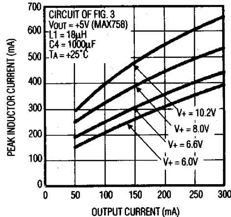
MAX738/MAX758 PEAK INDUCTOR CURRENT vs. OUTPUT CURRENT
