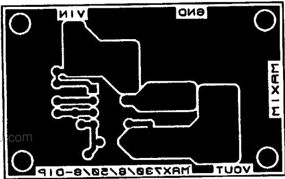
Figure 6. DIP PC Layout, Solder Side (1X Scale)
