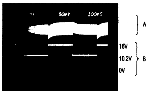
MAX738/MAX758 LINE-TRANSIENT RESPONSE
