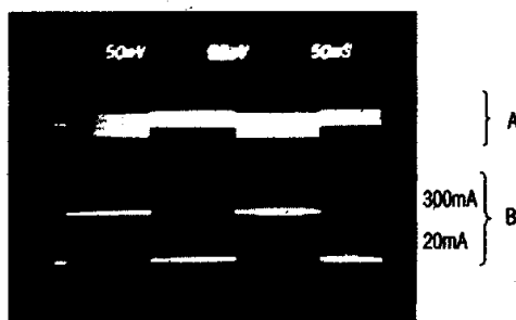
MAX730/MAX750 LOAD-TRANSIENT RESPONSE
