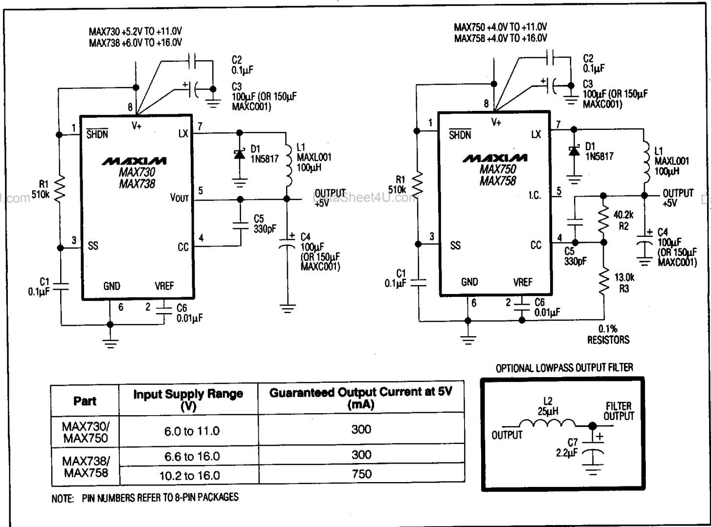
Figure 3. Standard +5V Step-Down Application Circuit
