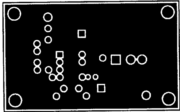
Figure 5. DIP PC Layout, Component Side (1X Scale)
