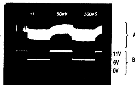
MAX730/MAX750 LINE-TRANSIENT RESPONSE
