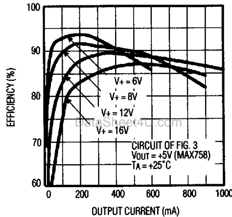
MAX738/MAX758 EFFICIENCY vs. OUTPUT CURRENT
