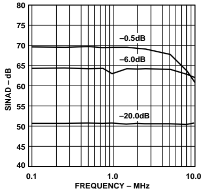
Figure 14. SINAD vs. Input Frequency (Input Span = 2.0 V p-p, V_{CM} = 2.5 V)
