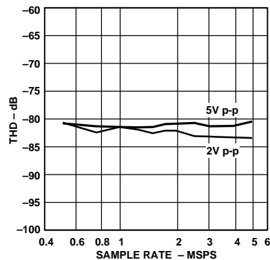
Figure 18. THD vs. Sample Rate ( A_{IN} = -0.5 dB, f_{IN} = 500 kHz, V_{CM} = 2.5 V)
