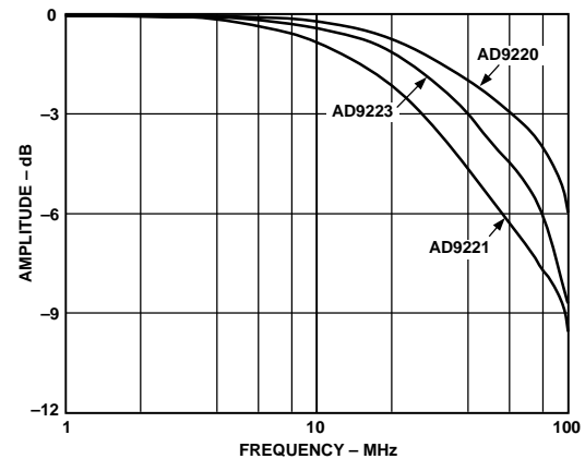
Figure 29. Full-Power Bandwidth
