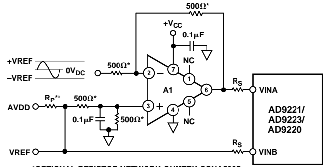
*OPTIONAL RESISTOR NETWORK-OHMTEK ORNA500D **OPTIONAL PULL-UP RESISTOR WHEN USING INTERNAL REFERENCE
