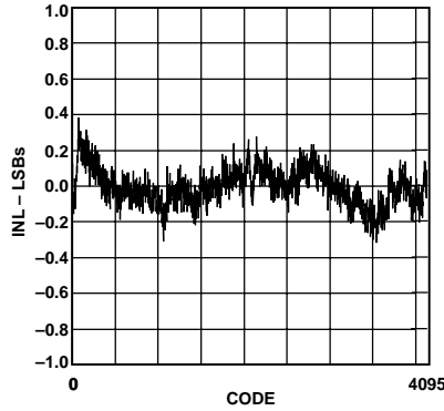
Figure 12. Typical INL
