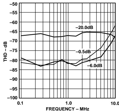
Figure 15. THD vs. Input Frequency (Input Span = 2.0 V p-p, V_{CM} = 2.5 V)
