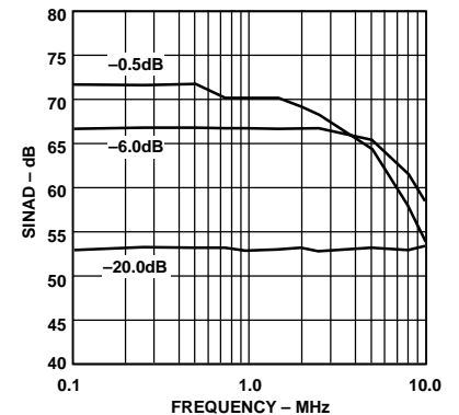
Figure 16. SINAD vs. Input Frequency (Input Span = 5.0 V p-p, V_{CM} = 2.5 V)
