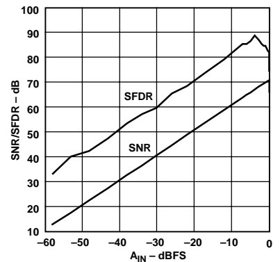
Figure 19. SNR/SFDR vs. A_{IN} (Input Amplitude) ( f_{IN} = 1.5 MHz, Input Span = 2 V p-p, V_{CM} = 2.5 V)
