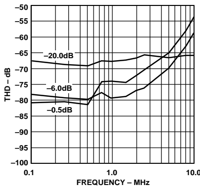
Figure 17. THD vs. Input Frequency (Input Span = 5.0 V p-p, V_{CM} = 2.5 V)
