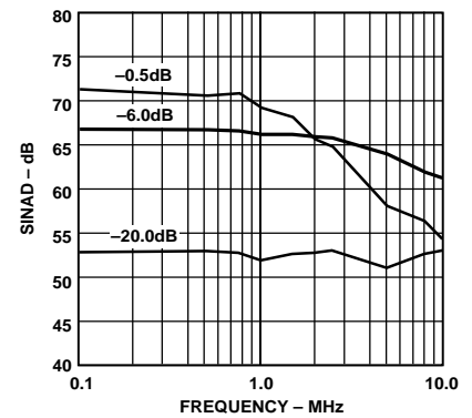
Figure 25. SINAD vs. Input Frequency (Input Span = 5.0 V p-p, V CM = 2.5 V)
