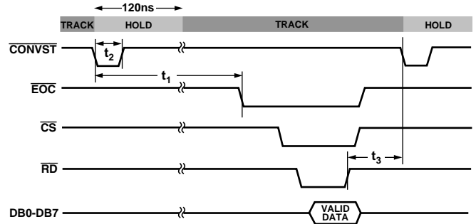
Figure 4. Track-and-Hold Timing
