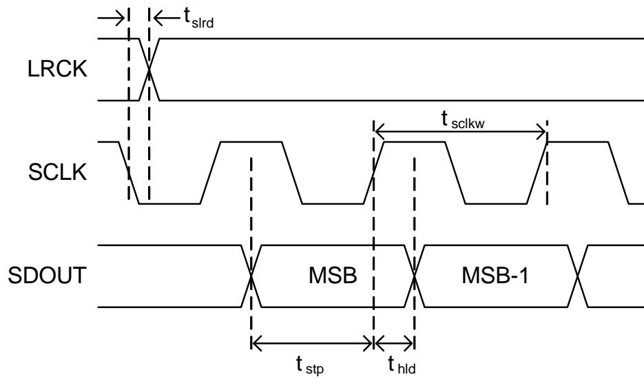
Figure 1. CS5343 I 2 S Serial Audio Interface
