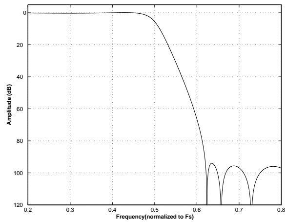
Figure 36. DAC Quad-Speed (fast) Transition Band
