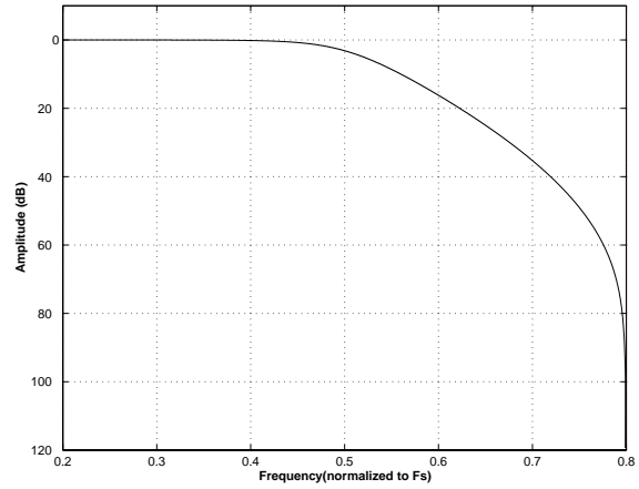
Figure 32. DAC Double-Speed (slow) Transition Band
