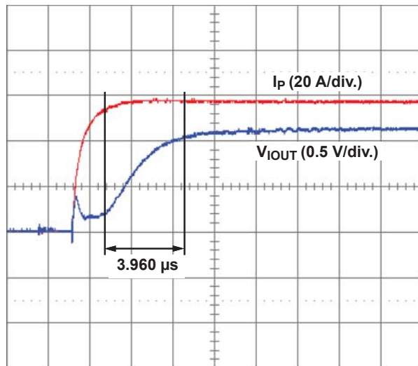
Response Time
