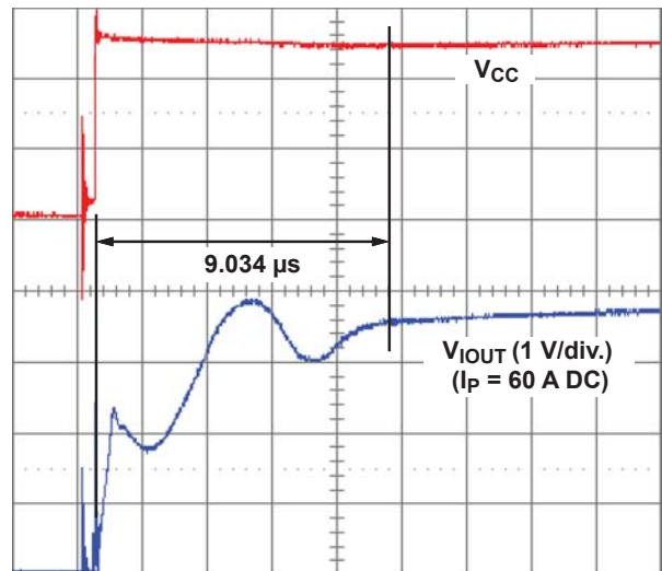
Power-on Delay
