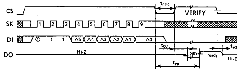
Figure 12 ERASE Timing (S-29130A)
