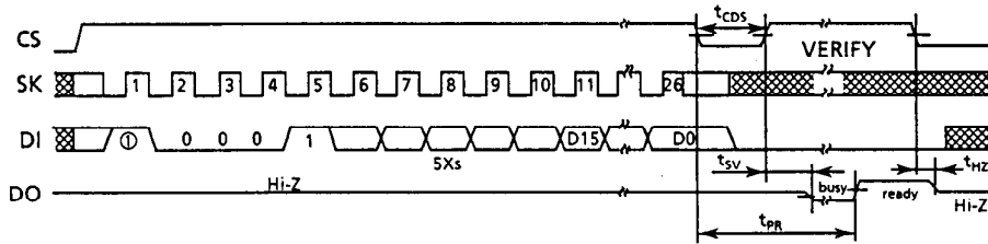
Figure 17 WRAL Timing (S-29230A)
