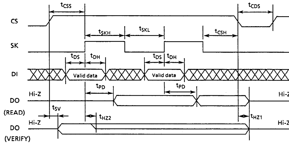
Figure 3 Timing Chart
