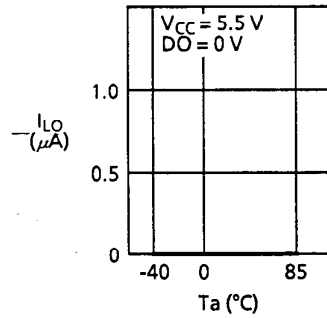
1.13 Output leakage current I_{LO} - Ambient temperature T_a
