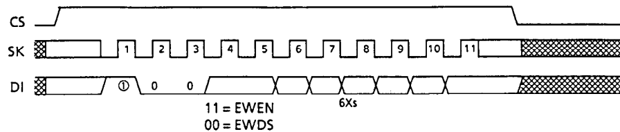
Figure 27 EWEN/EWDS Timing (S-29330A)
