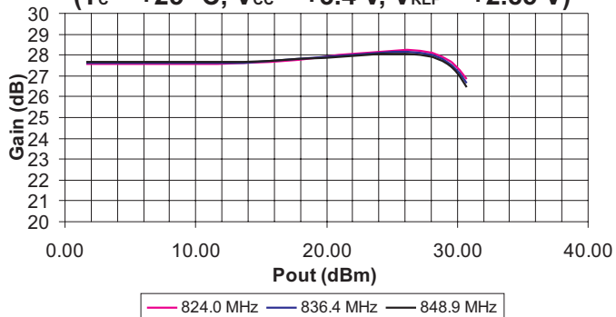
Figure 11: Large Signal Gain vs. Output Power Over Frequency
