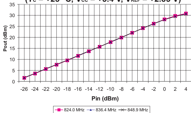
Figure 9: Input Power vs. Output Power Over Frequency
