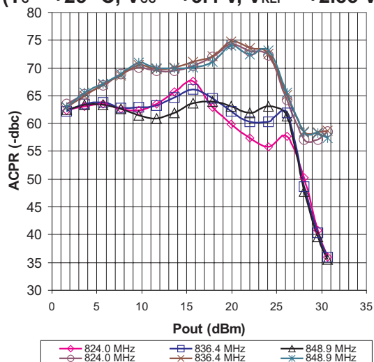
Figure 10: ACP1 and ACP2 vs. Output Power Over Frequency
