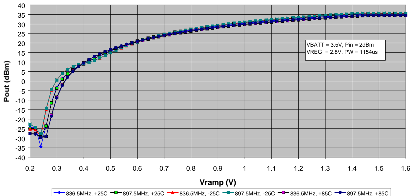
Figure 3: GSM850/GSM900 Pout vs Vramp & Temperature (2 TX slots)
