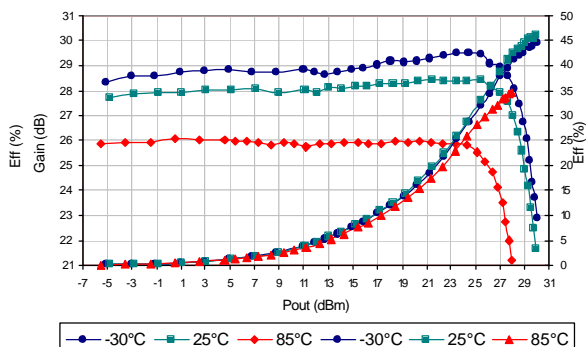
Figure 26 IS-98D Gain & Eff. versus Pout @ 836.5 MHz Vcc: 3.5V, Vref: 3.0V, Vmode: 0.0V
