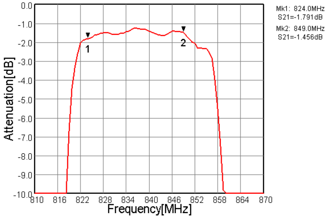
Fig.3 In-band Characteristics
