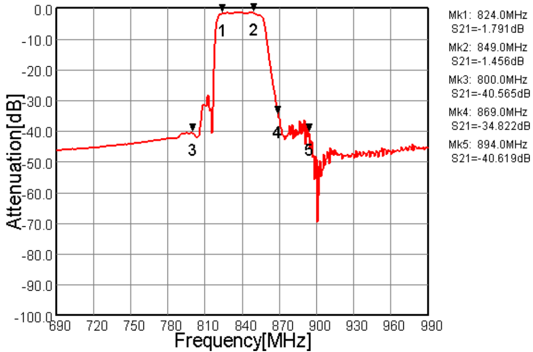
Fig.1 Pass-band Characteristics
