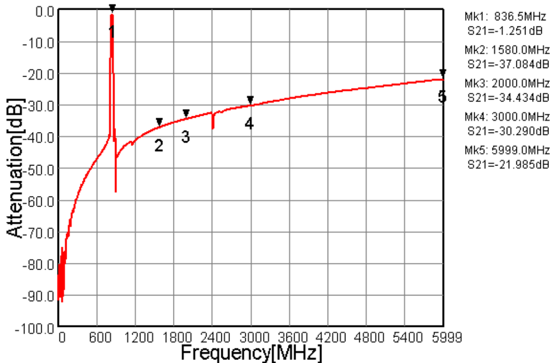
Fig.4 Wide-band Characteristics
