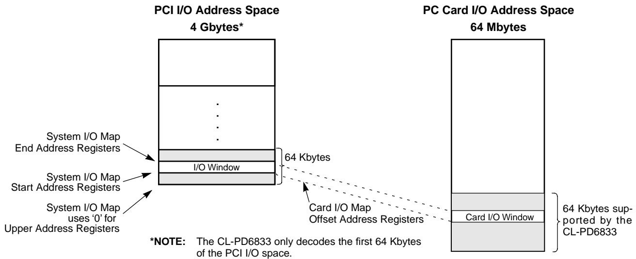
Figure 3-2. R2 I/O-to-I/O Window Organization
