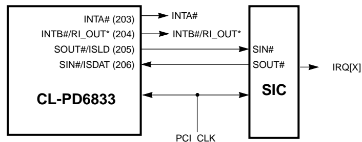
Figure 3-9. PC/PCI Serial Interrupt Signalling Mode
