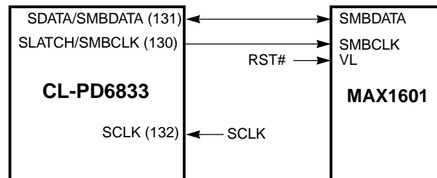
Figure 3-12. Power Control Using SMBus Signalling Mode
