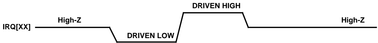
Figure 11-1. Pulse Mode Interrupts
