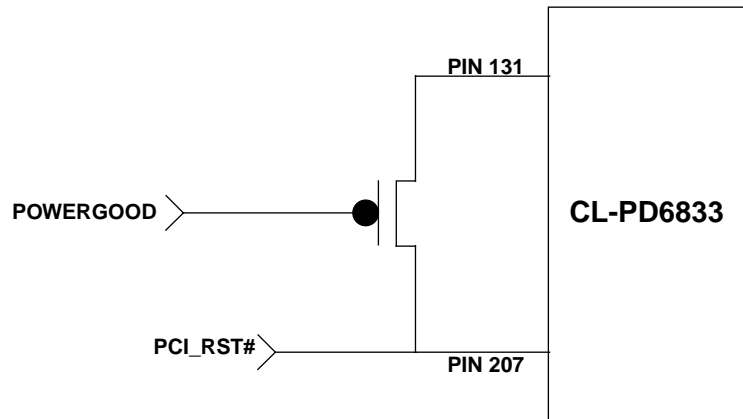
Figure 3-13. Power-on Detection for Power Management
