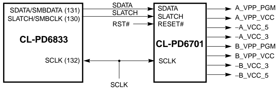
Figure 3-11. Power Control Using External-Hardware Signalling Mode
