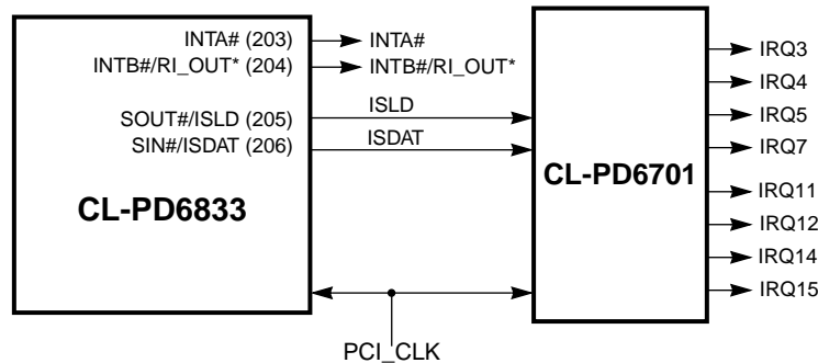
Figure 3-6. External-Hardware Interrupt Signalling Mode
