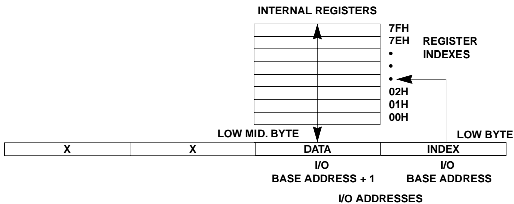
Figure 3-14. Indexed 8-Bit Register Structure
