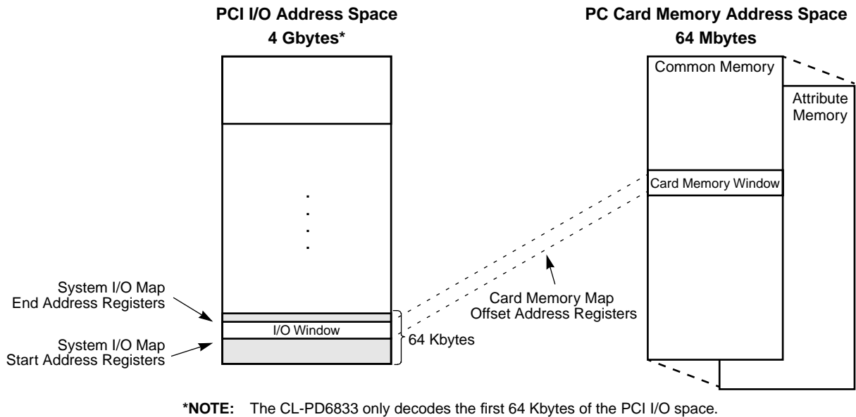
Figure 3-4. R2 I/O-to-Memory Window Organization
