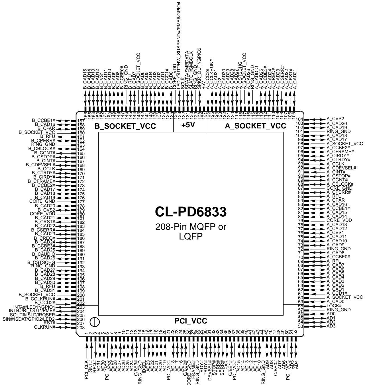
Figure 2-2. Pin Diagram for PC Card 32 (CardBus)
