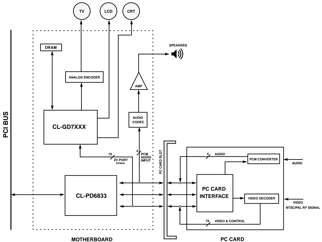
Figure 3-5. A Typical ZV Port Implementation
