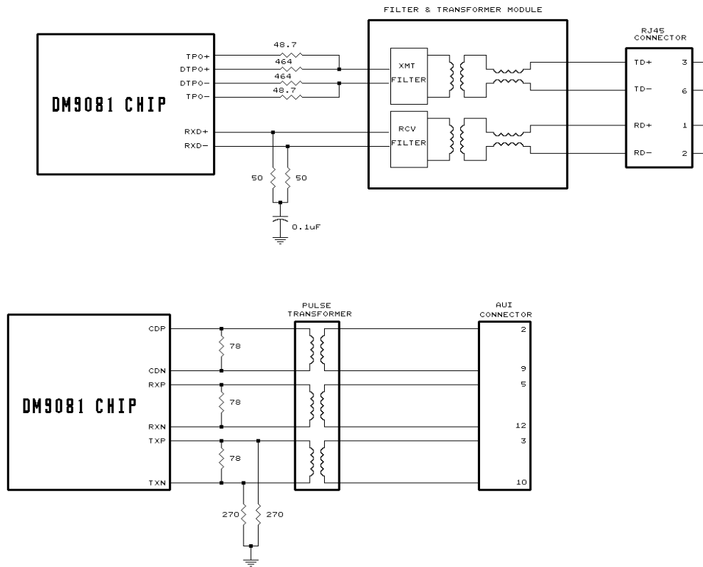
Figure 6. Typical Single AUI Port Using Components
