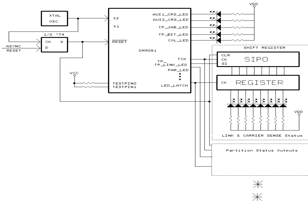
Figure 4. Normal Mode Implementation
