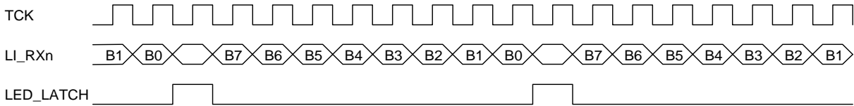
Figure 3. Serial LED Signal Timing
