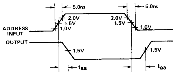
FIGURE 1: Access Time Via Address Input
