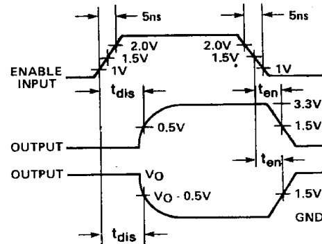
FIGURE 2: Output Disable And Enable Time
