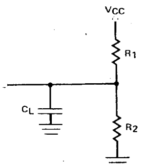
FIGURE 4: Output Load Circuit
