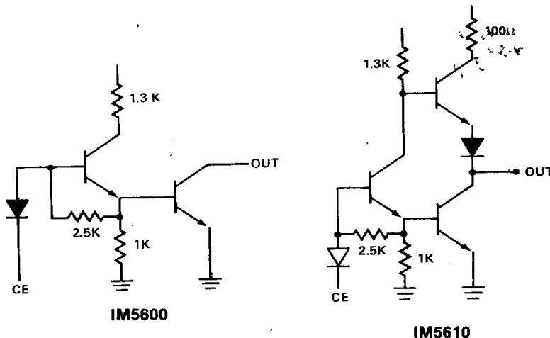
FIGURE 3: Output Stage Schematics
