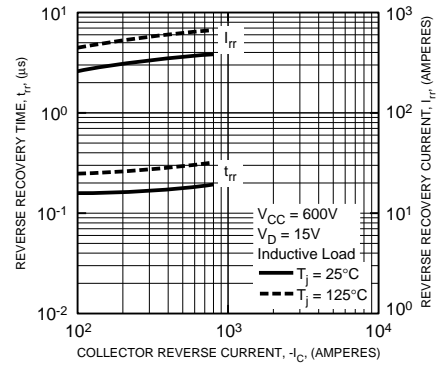
REVERSE RECOVERY CURRENT VS. COLLECTOR CURRENT (TYPICAL)
