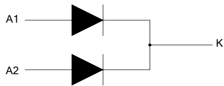
Figure 3. Internal Structure of MBR20H100C
