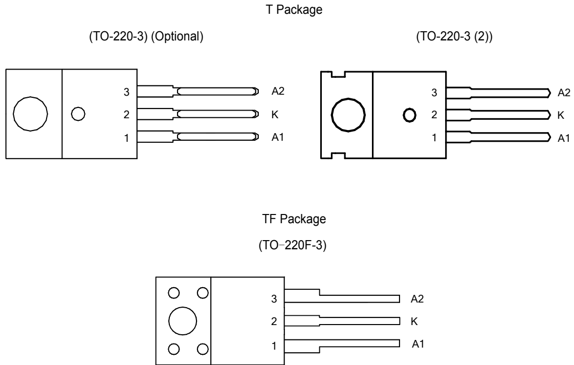
Figure 2. Pin Configuration of MBR20H100C (Top View)
