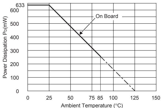
Power Dissipation
