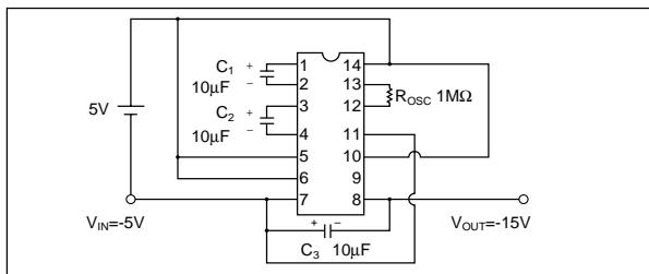
Voltage Tripler
