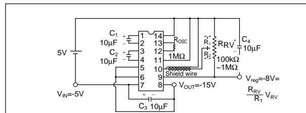
Tripler+Regulator (-0.4%/°C selected as temperature gradient)
