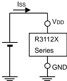
Nch Driver Output Current Test Circuit
