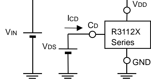
CD Pin Output Current Test Circuit
