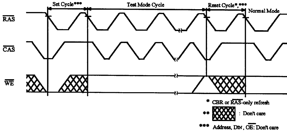
FIGURE 15. TEST MODE CYCLE
