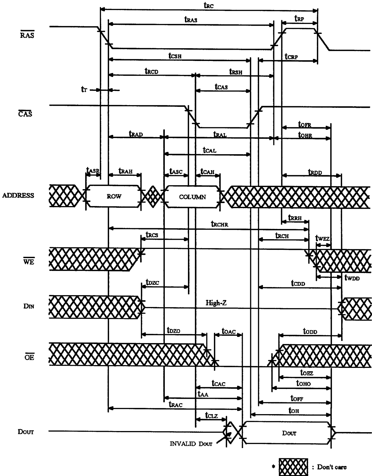
FIGURE 1. READ CYCLE
