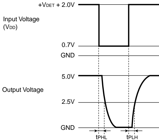
Nch Open Drain Output
