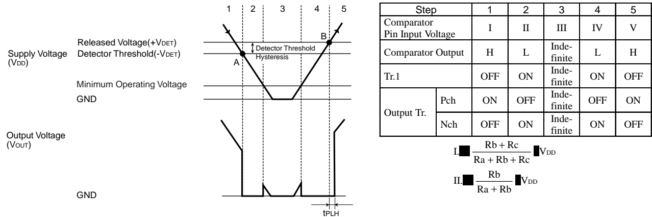
Figure 2. Operation Diagram
