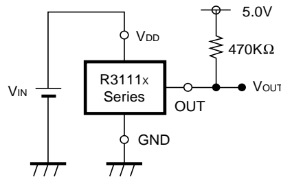
Figure 4. Detector Threshold Test Circuit
