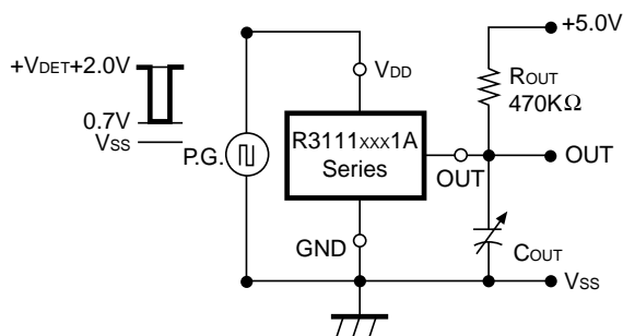
Figure 7. Output Delay Time Test Circuit (1)
