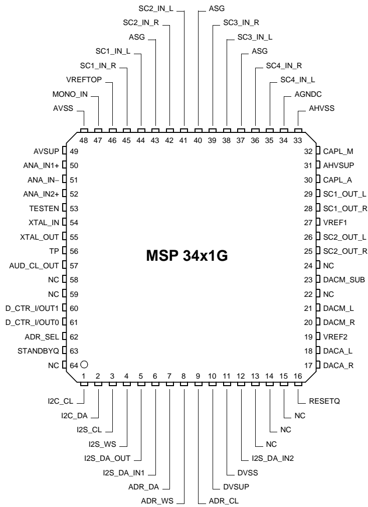
Fig. 4–10: 64-pin PLQFP package
