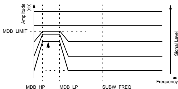
Fig. 2–5: Dynamic amplification
