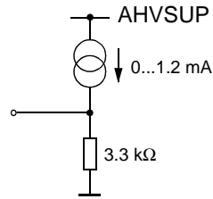
Fig. 4-21: Output Pins: DACA_R/L, DACM_R/L, DACM_SUB
