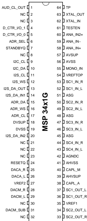
Fig. 4–7: 64-pin PSDIP package
