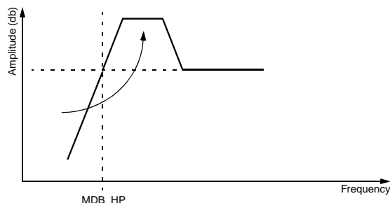
Fig. 2–6: Adding harmonics
