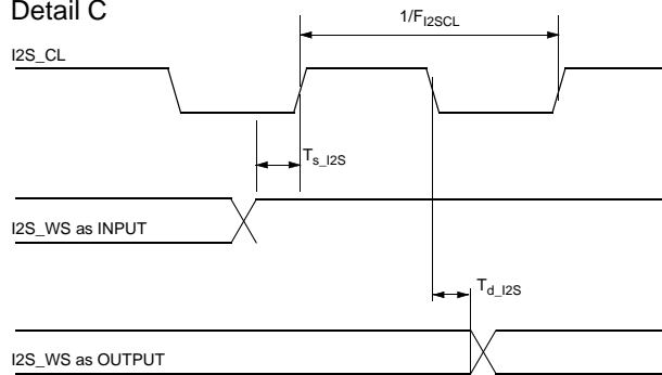
Fig. 4-28: I 2 S bus timing diagram
