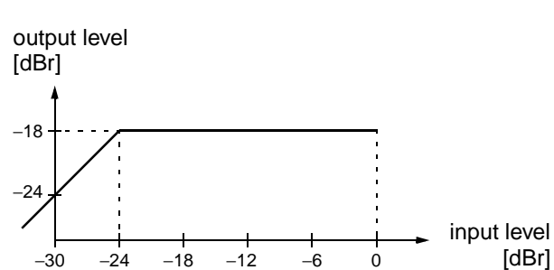
Fig. 2-4: Simplified AVC characteristics
