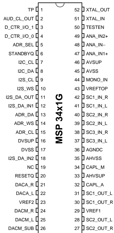
Fig. 4–8: 52-pin PSDIP package
