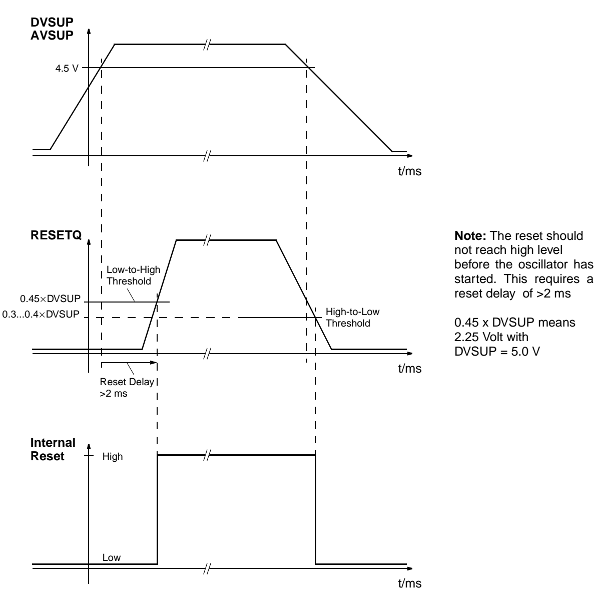
Fig. 4-26: Power-up sequence
