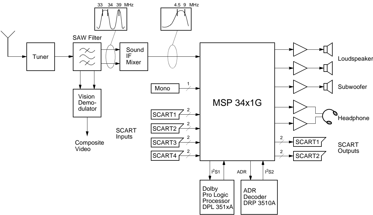
Fig. 1–2: Typical MSP 34x1G application
