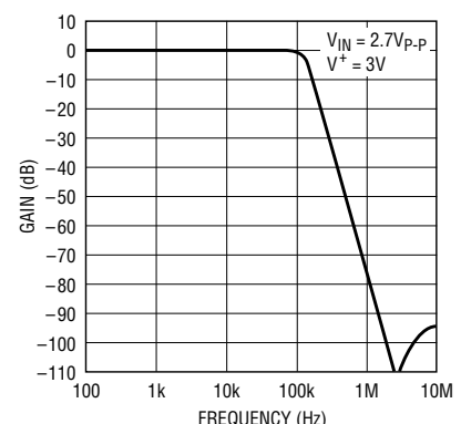
Frequency Response
