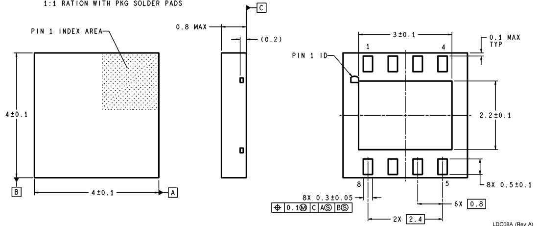
8-Pin LLP NS Package Number LDC08A
