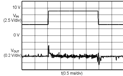
S-8520/1A30MC ( I_{OUT} :500 mA)
