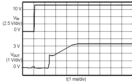
S-8520/1E33MC ( V_{IN} : 0 →9.0 V)
