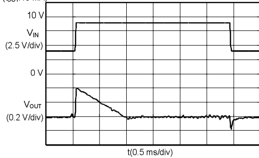
S-8520/1A30MC ( I_{OUT} :10 mA)
