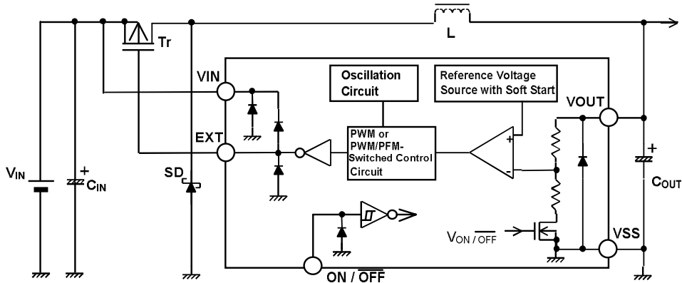
Figure 1 Block Diagram
