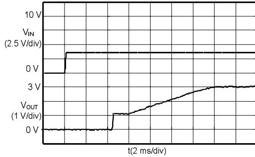
S-8520/1C30MC ( V_{IN} : 0 →3.6 V)
