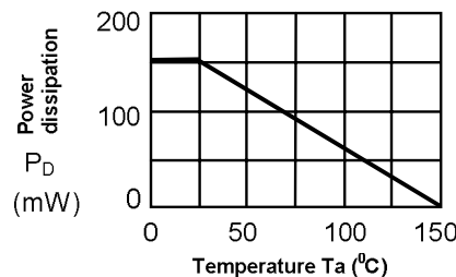
Figure 10 Power dissipation of an SOT-23-5 Package (Free-Air)
