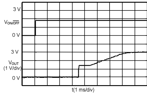
S-8520/1A30MC ( V_{IN} :3.6 V)
