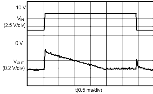
S-8520/1C33MC ( I_{OUT} :10 mA)
