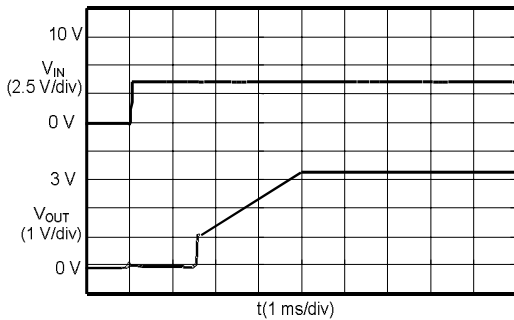
S-8520/1E33MC ( V_{IN} : 0 →4.0 V)
