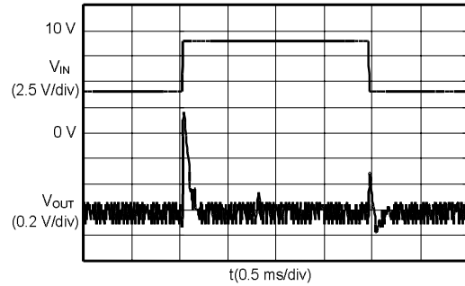
S-8520/1C33MC ( I_{OUT} :500 mA)
