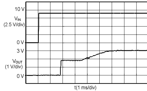
S-8520/1A30MC ( V_{IN} : 0 →9.0 V)
