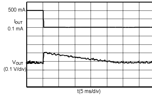
S-8520/1C30MC ( V_{IN} :3.6 V)
