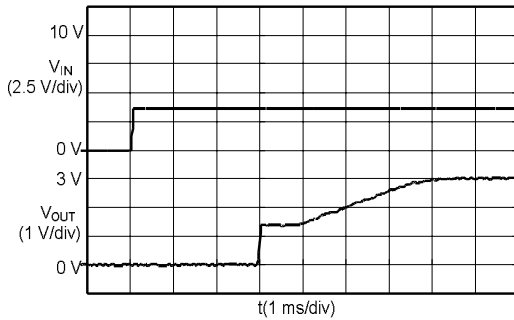
S-8520/1A30MC ( V_{IN} : 0 →3.6 V)
