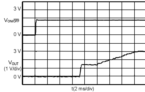
S-8520/1C30MC ( V_{IN} :9.0 V)
