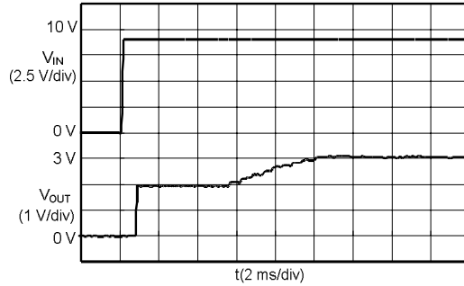
S-8520/1C30MC ( V_{IN} : 0 →9.0 V)
