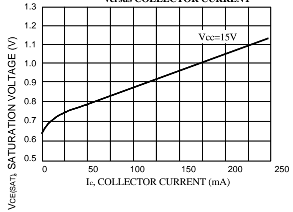
FIGURE 6 – COMMON-EMITTER CONFIGURATION OUTPUT-SATURATION VOLTAGE versus COLLECTOR CURRENT
