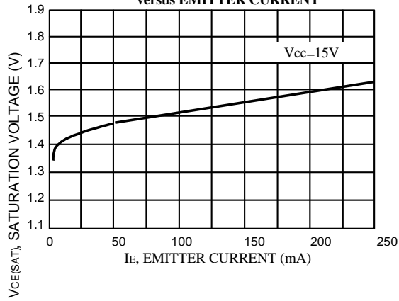
FIGURE 5 – EMITTER-FOLLOWER CONFIGURATION OUTPUT-SATURATION VOLTAGE versus EMITTER CURRENT
