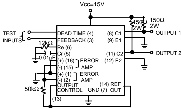
TEST CIRCUIT
