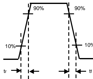
OUTPUT VOLTAGE WAVEFORM
