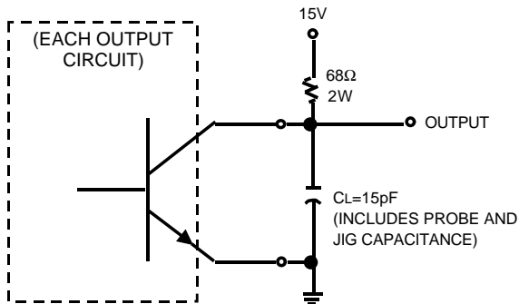
TEST CIRCUIT
