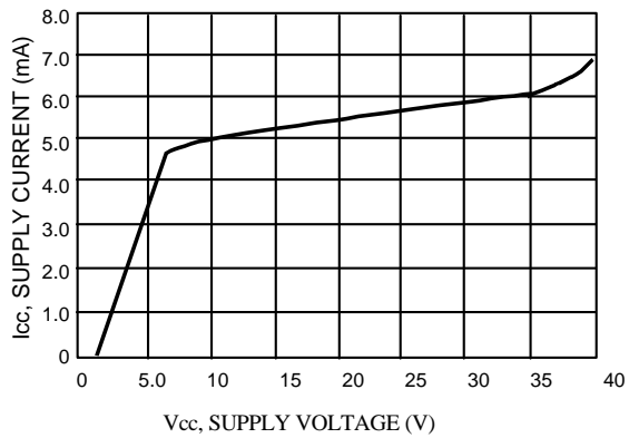
FIGURE 7 – STANDBY-SUPPLY CURRENT versus SUPPLY VOLTAGE
