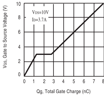
Figure 9. Gate Charge
