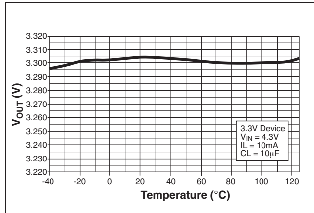
Figure 10. Output Voltage vs Temperature at I_{LOAD}=10mA
