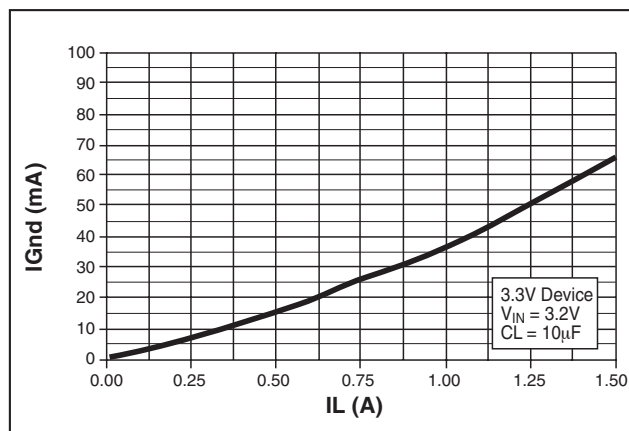
Figure 7. Ground Current vs Load Current in Dropout
