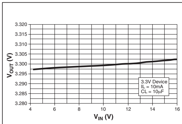
Figure 3. Line Regulation for 3.3V Device
