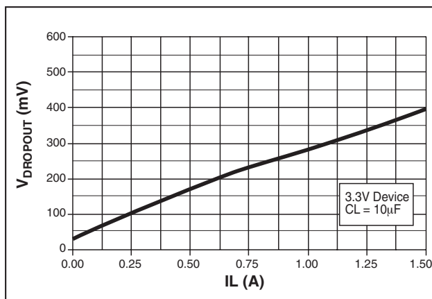
Figure 8. Dropout Voltage vs Load Current for 3.3V Device
