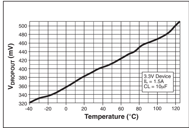
Figure 16. Dropout Voltage vs Temperature at I_{LOAD}=1.5A
