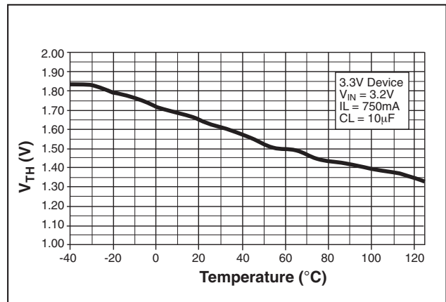
Figure 18. Enable Threshold vs Temperature for 3.3V Devices
