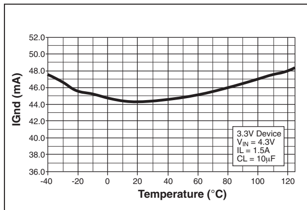
Figure 13. Ground Current vs Temperature at I_{LOAD}=1.5A
