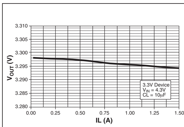
Figure 4. Load Regulation for 3.3V Device
