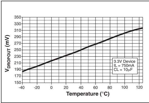
Figure 15. Dropout Voltage vs Temperature at I_{LOAD}=750mA
