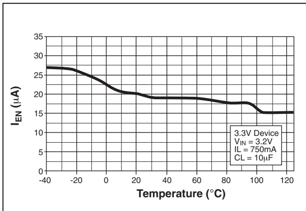
Figure 17. Enable Current vs Temperature for 3.3V Devices
