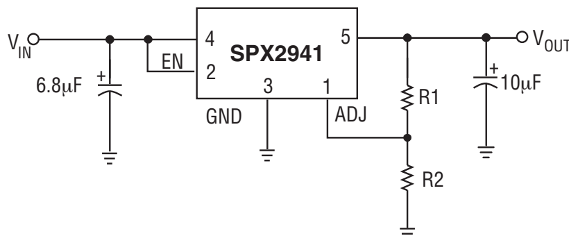
Figure 1. Adjustable Output Linear Regulator
