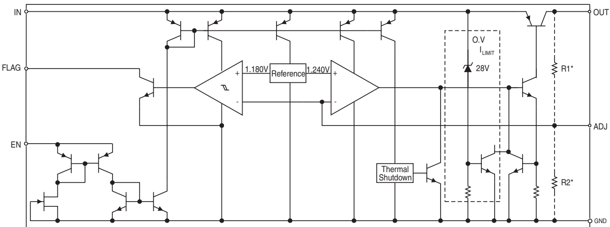
Figure 2. SP2941 Block Diagram
