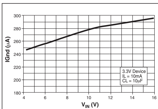
Figure 6. Ground Current vs Input Current
