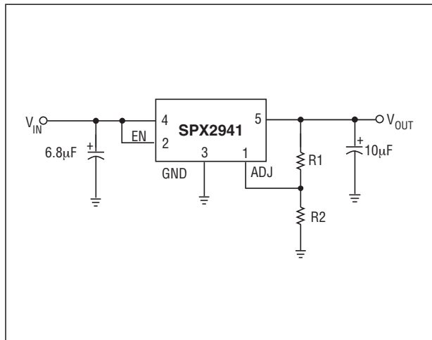
Figure 19. Adjustable Output Linear Regulator
