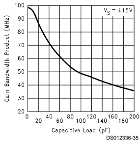
Gain Bandwidth Product vs Load Capacitance
