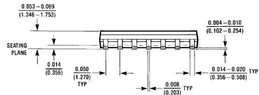
14-Pin Small Outline Package Order Number LM6144AIM or LM6144BIM NS Package Number M14A
