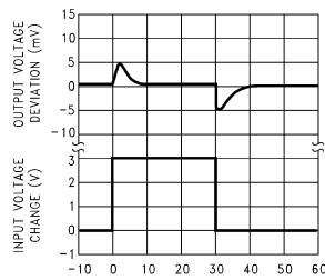
Line Transient Response ( V_{buf} )
