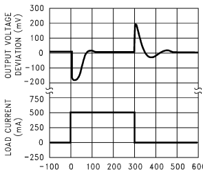
Load Transient Response ( V_{OUT} )
