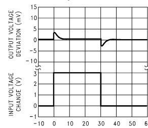
Line Transient Response ( V_{stby} )
