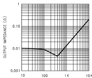
Output Impedance ( V_{OUT} )
