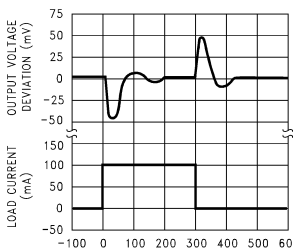
Load Transient Response ( V_{buf} )
