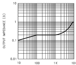
Output Impedance ( V_{buf} )
