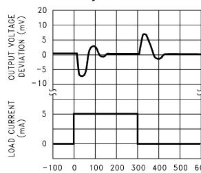
Load Transient Response ( V_{stby} )
