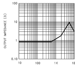
Output Impedance ( V_{stby} )
