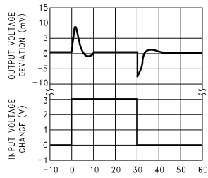
Line Transient Response ( V_{OUT} )
