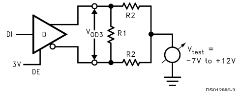
FIGURE 5. V_{OD3}
