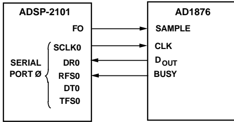
Figure 8. ADSP-2101 Interface
