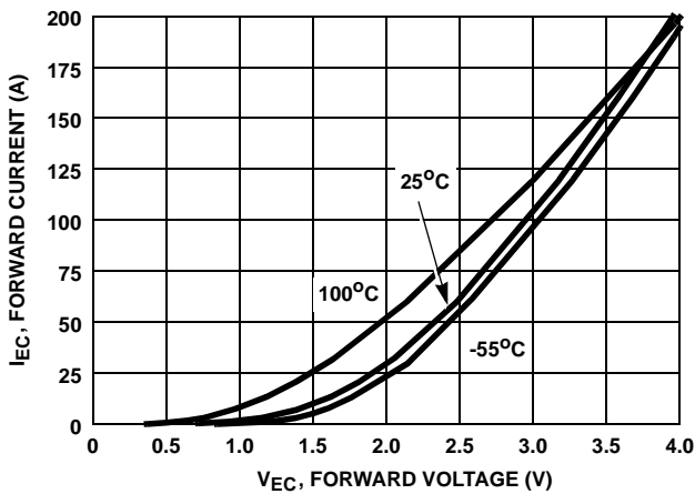
FIGURE 17. DIODE FORWARD CURRENT vs FORWARD VOLTAGE DROP
