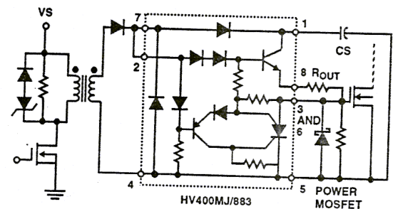
FIGURE 1. UNIPOLAR DRIVE
