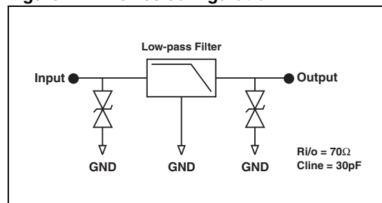
Figure 2. Device configuration
