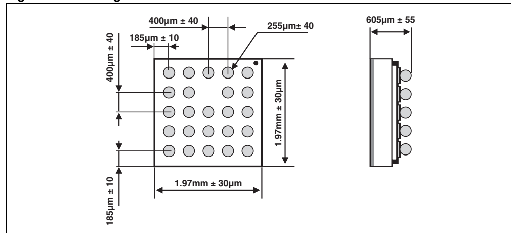
Figure 11. Package dimensions
