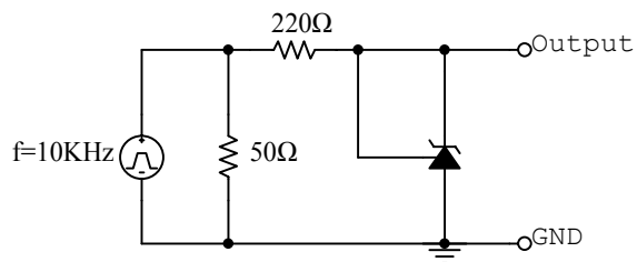
Fig.11 Test circuit for Fig. 10
