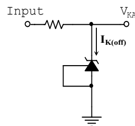
Fig. 3 Test circuit for I_{K(off)}
