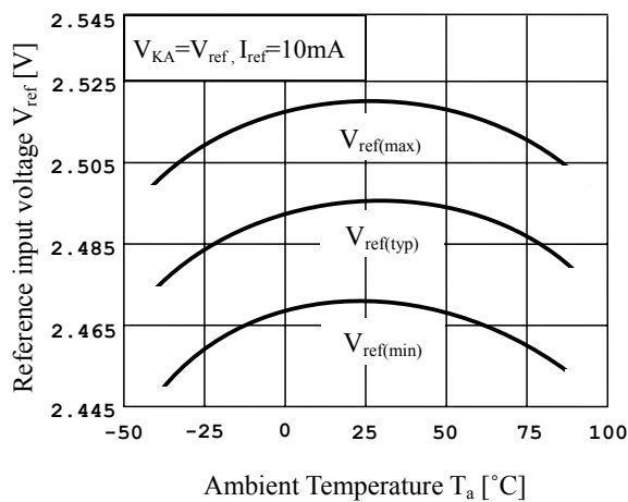
Fig.8 V_{ref} vs T_a
