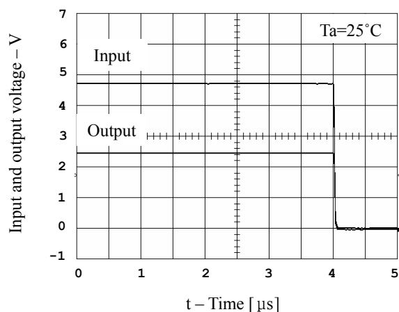
Fig.13 Pulse Response (Magnify B of Fig.10)
