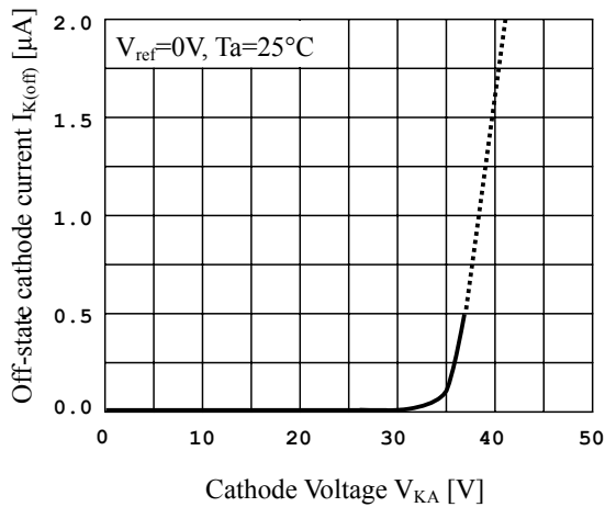
Fig.6 I_{K(off)} vs V_{KA}
