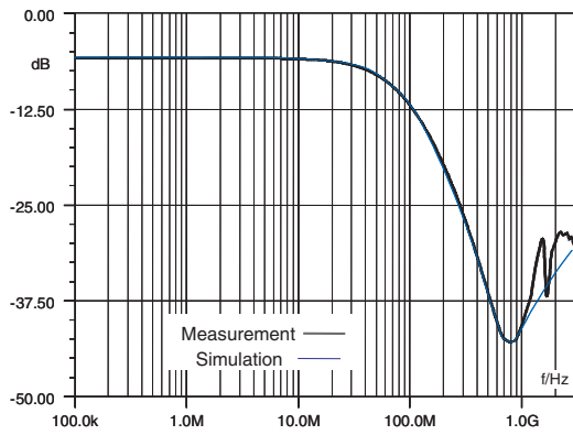
Figure 5: Digital crosstalk measurements
