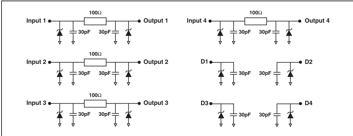
Figure 2: Basic Cell Configuration
