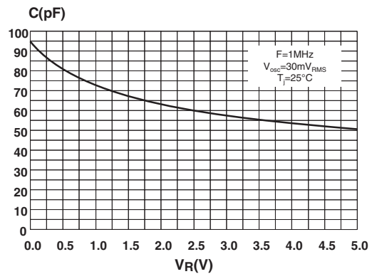
Figure 8: Line capacitance versus applied voltage for filter
