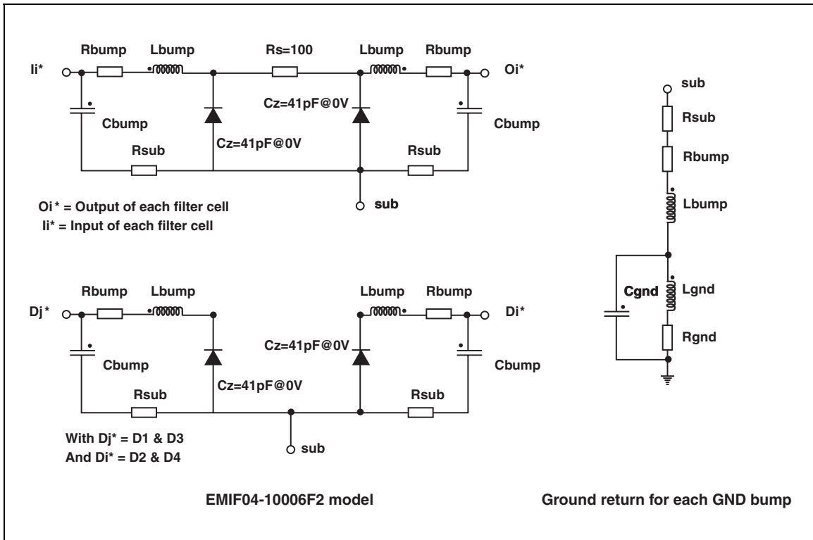
Figure 9: Aplac model
