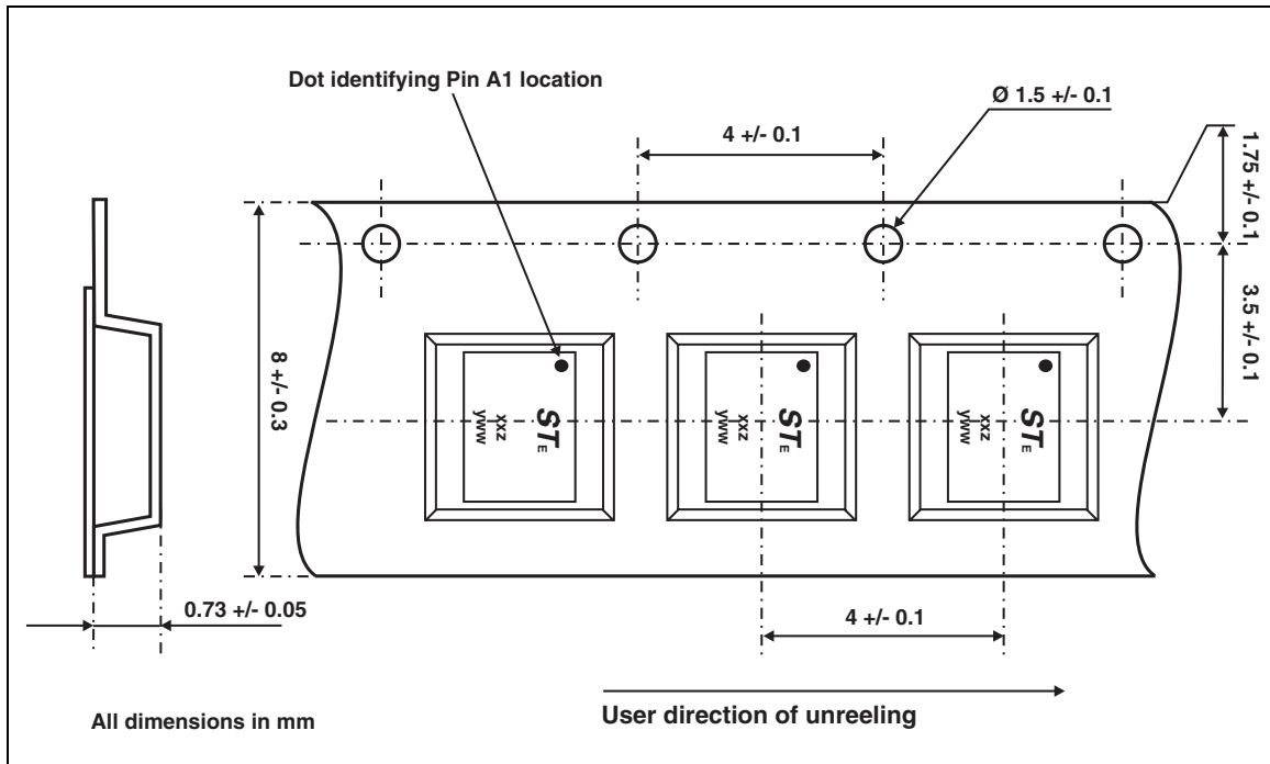
Figure 15: FLIP-CHIP Tape and Reel Specification
