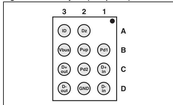
Figure 1. Pin layout (bump side)
