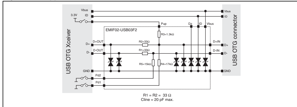
Figure 9. Aplac model
