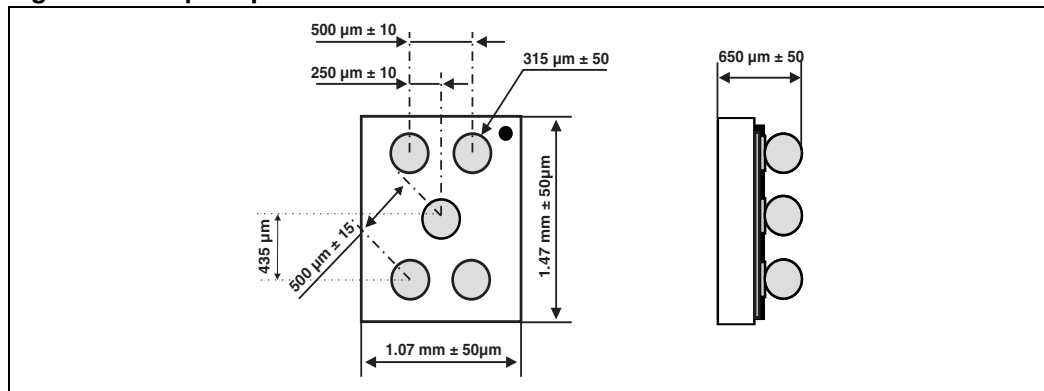
Figure 12. Flip-Chip dimensions
