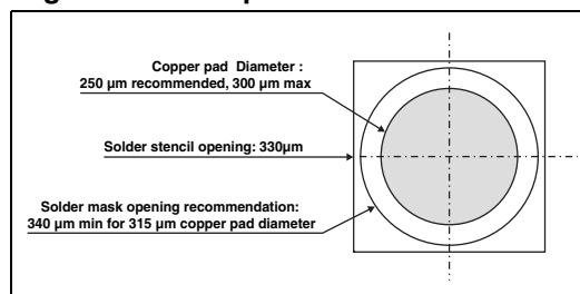
Figure 13. Footprint
