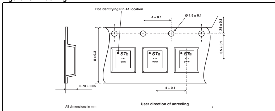
Figure 15. Packing
