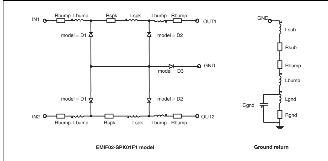
Figure 9. Aplac mode
