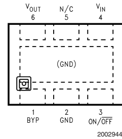
6-Lead LLP Package (LD)
