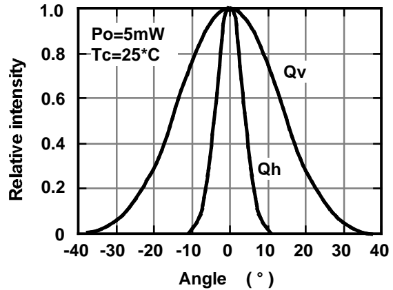
Beam divergence
