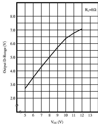
V_{CC} – Maximum Output Amplitude Characteristics
