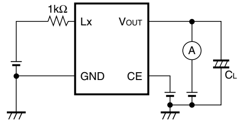
Test Circuit 2
