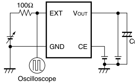
Test Circuit 4
