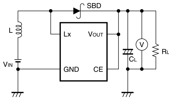
Test Circuit 1
