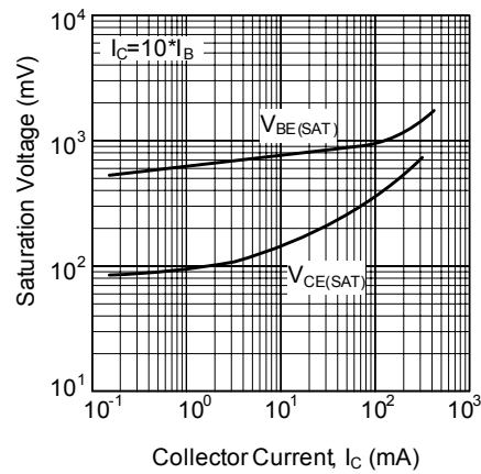
Fig.4 Saturation Voltage
