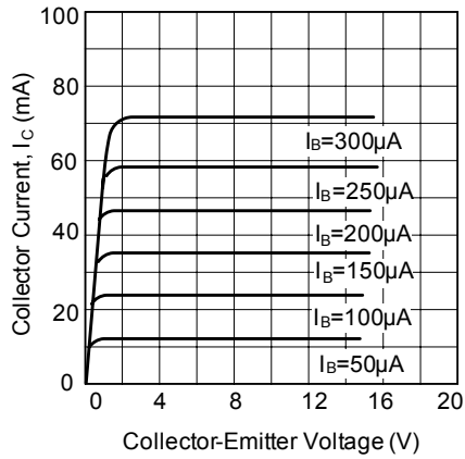
Fig.1 Static characteristics
