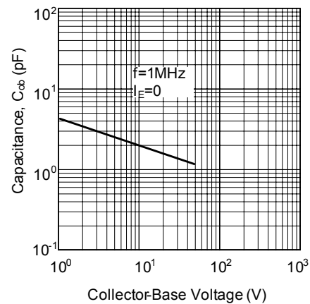
Fig.6 Collector Output Capacitance
